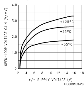
Gain vs Supply Voltage
