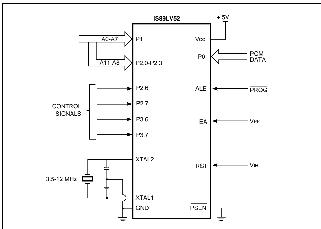
Figure 27. Programming the Flash Memory
