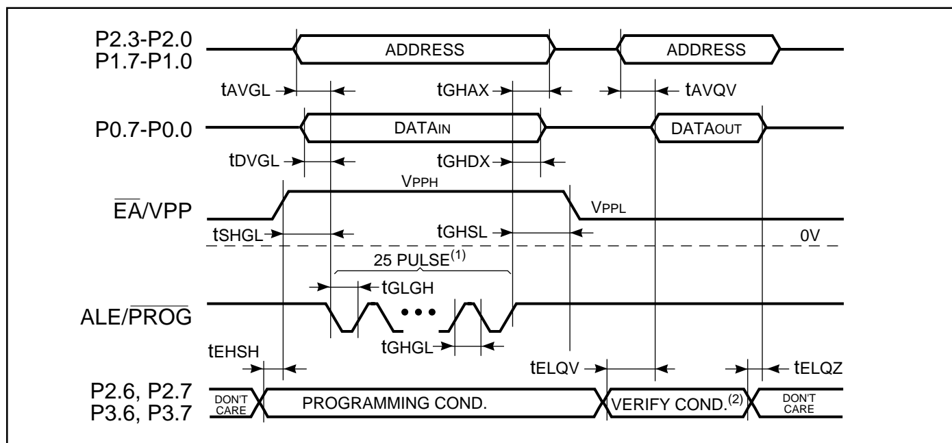
Figure 29. Flash Memory Programming and Verification Timing Waveform
