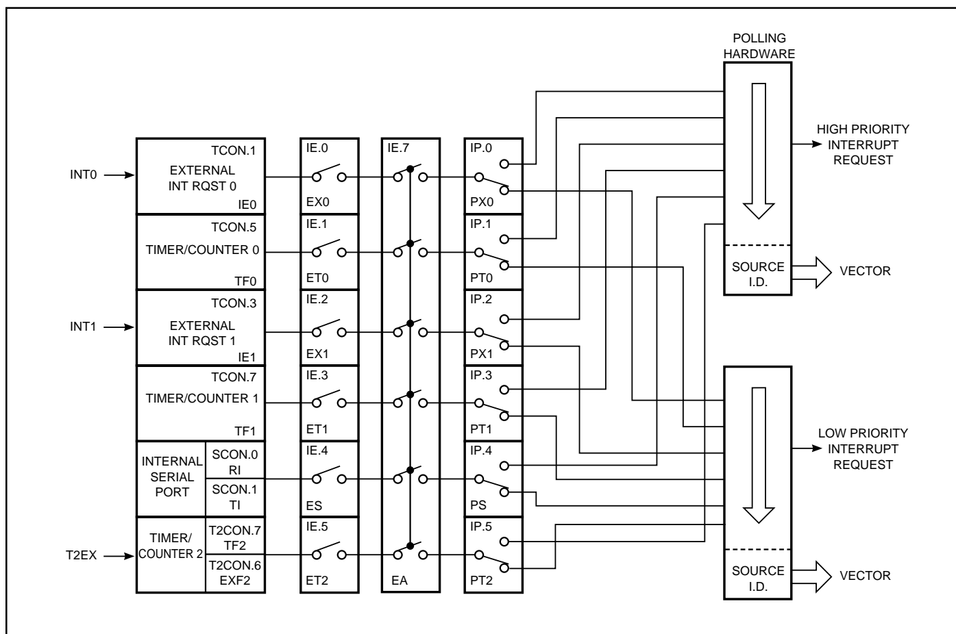
Figure 19. Interrupt System
