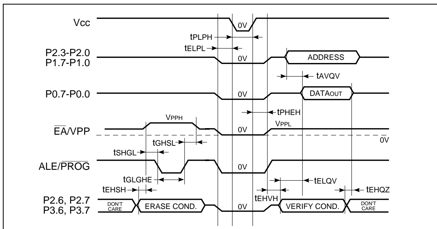
Figure 30. Flash Memory Erase Timing Waveform
