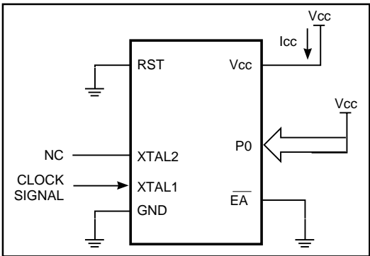
Figure 32. Idle Mode
