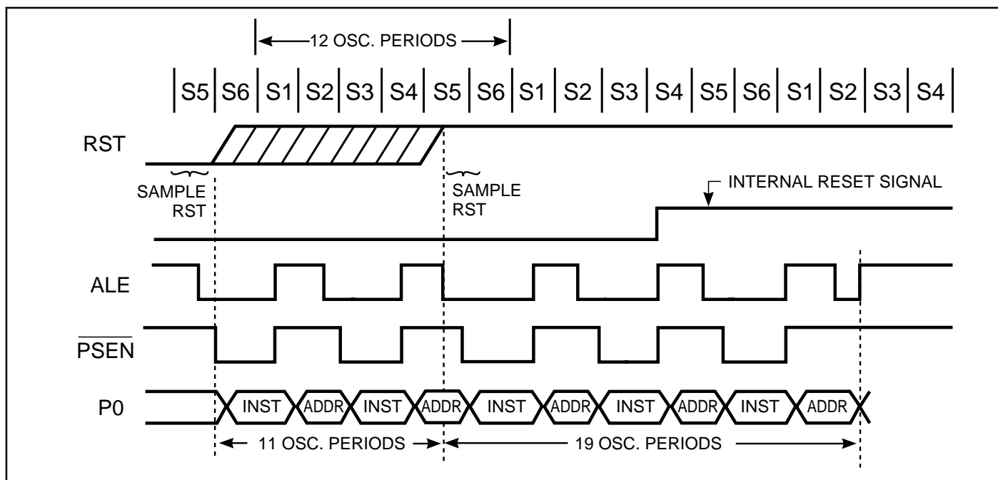
Figure 21. Reset Timing
