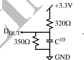
Figure B: 3.3V Output load
