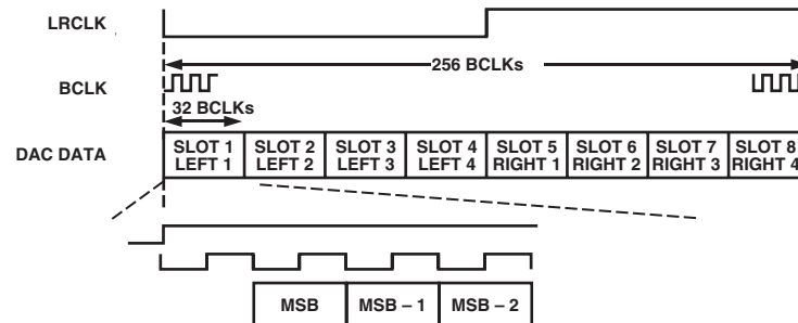
Figure 8b. DAC Packed Mode 256
