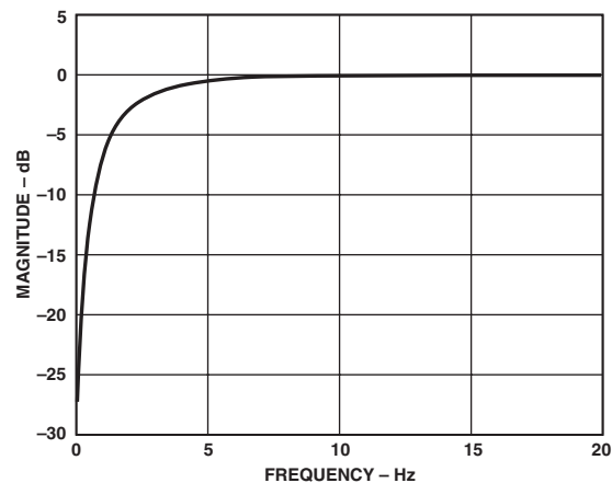
TPC 2. ADC High-Pass Filter Response, f_s = 48 \text{ kHz}
