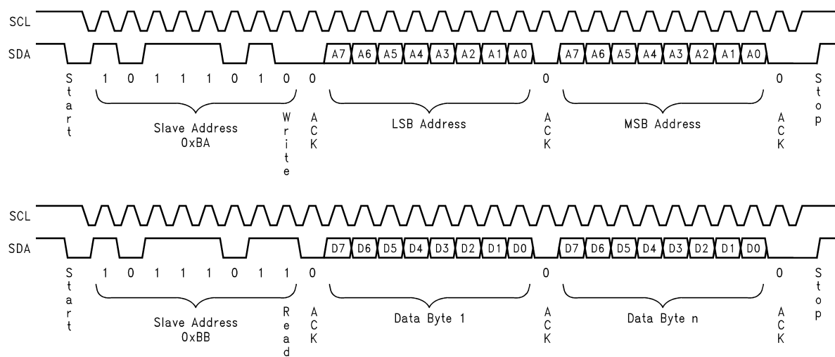
FIGURE 16. I²C Compatible Read Sequence
