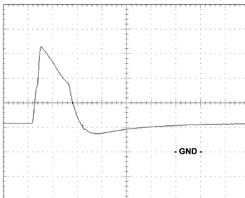
FIGURE 4. Deflection Horizontal Blanking
