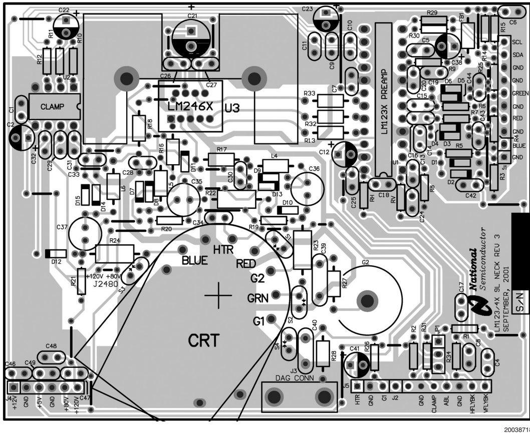
FIGURE 11. LM123x-LM246x Demo Board Layout
