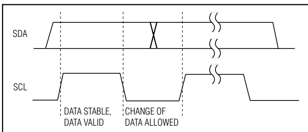
Figure 4. Bit Transfer
