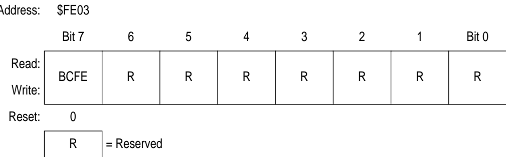
Figure 22-7. SIM Break Flag Control Register (SBFCR)
