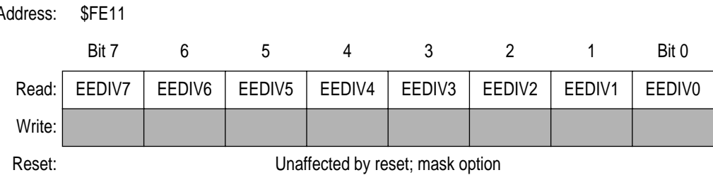
Figure 5-8. EEPROM Divider Mask Option Register Low (EEDIVLMOR)
