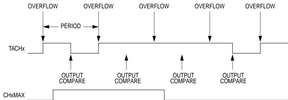
Figure 11-13. CHxMAX Latency
