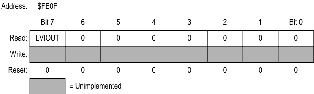
Figure 21-3. LVI Status Register (LVISR)
