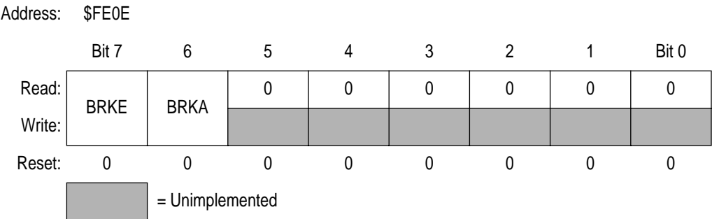
Figure 22-3. Break Status and Control Register (BRKSCR)
