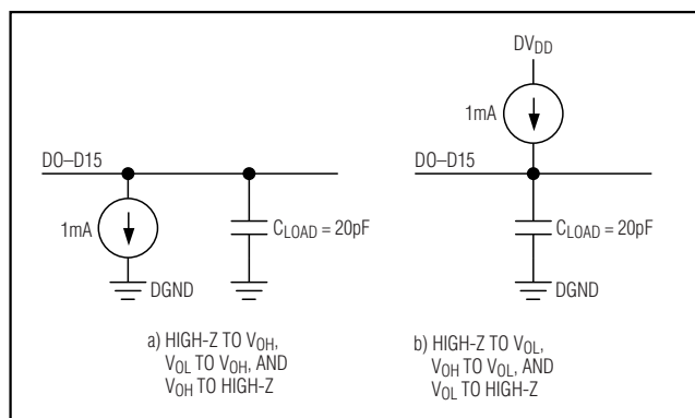
Figure 1. Load Circuits
