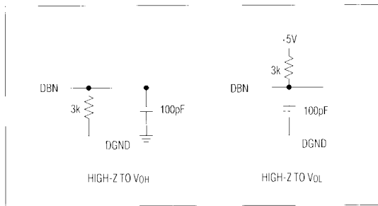
Figure 3. Load Circuits for Access Time Test ( t_{11} )
