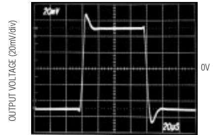
TIME (20 \mu s/div) A_V = +1, C_L = 15\text{pF}
