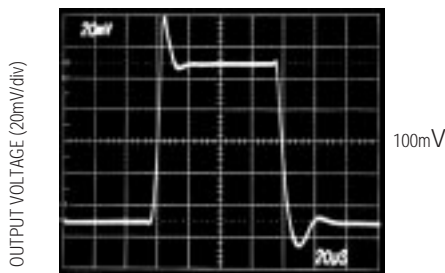
TIME (20 \mu s/div) A_V = +1, C_L = 15\text{pF}
