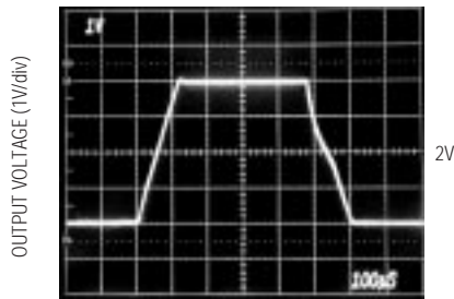
TIME (100 \mu s/div) A_V = +1, C_L = 15\text{pF}
