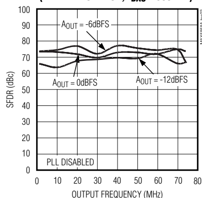
SPURIOUS-FREE DYNAMIC RANGE vs. OUTPUT FREQUENCY (4x INTERPOLATION, f_{DAC} = 165MHz )
