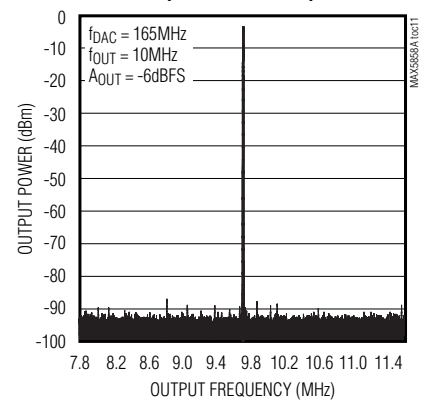
FFT PLOT (±2MHz WINDOW)
