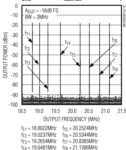
8-TONE MTPR PLOT (NO INTERPOLATION, f_{DAC} = 165MHz , f_{CENTER} = 19.9503MHz )
