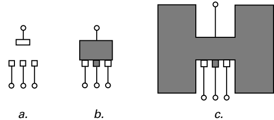
Figure 4. PCB Layouts
