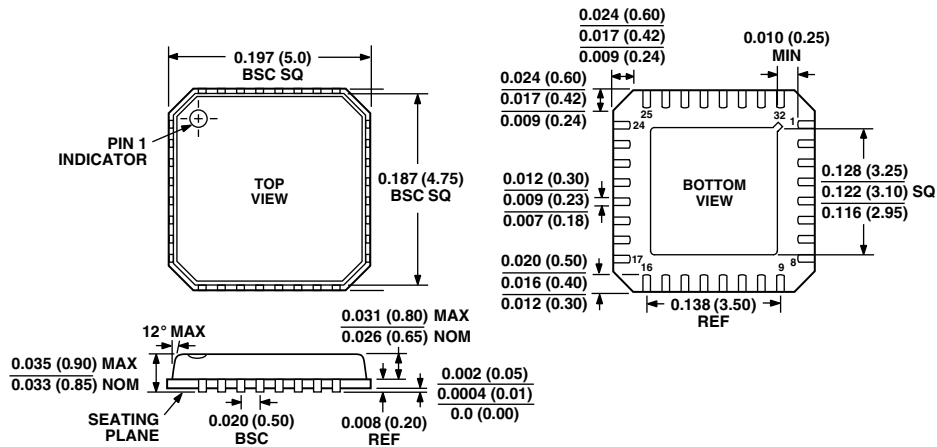
32-Lead LFCSP (CP Suffix)
