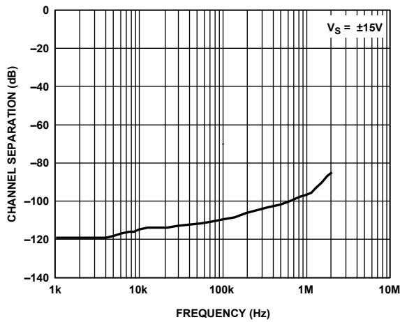
Figure 27. Channel Separation
