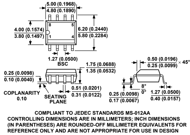
Figure 58. 8-Lead Small Outline IC [SOIC] (R-8)—Dimensions shown in millimeters
