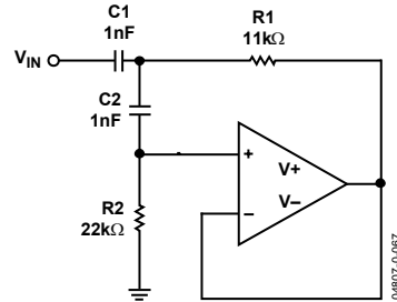
Figure 56. Two Pole High-Pass Filter
