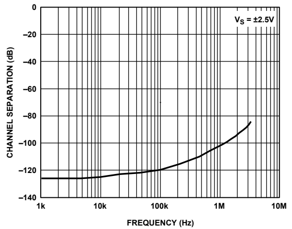
Figure 48. Channel Separation
