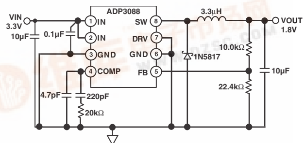
Figure 1. Typical Application
