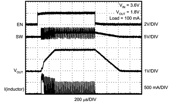
Shutdown Response (PWM Mode)
