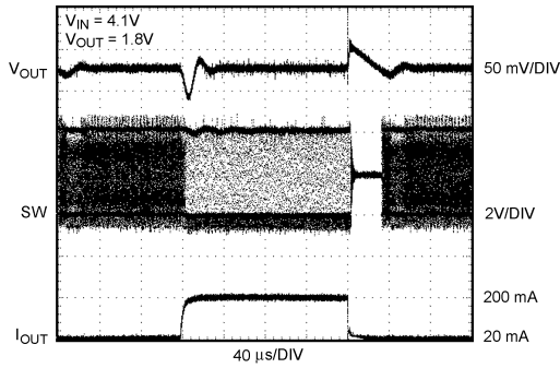
Load Transient Response (PWM Mode)
