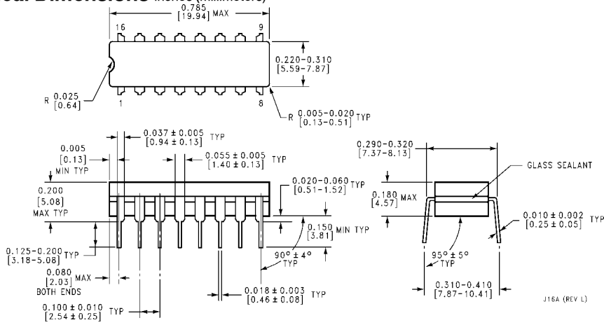
Ceramic Dual-In-Line Package (J) Order Number CD4028BMJ or CD4028BCJ NS Package Number J16A
