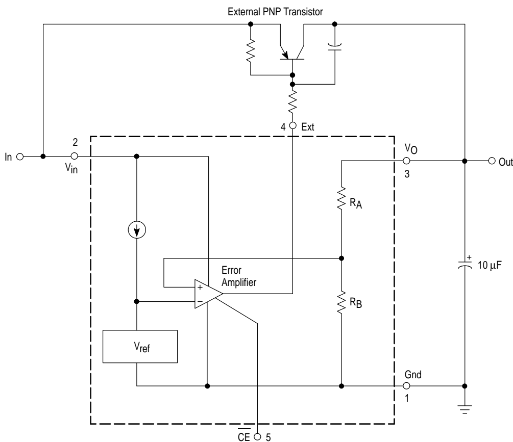
Figure 9. Typical Operation
