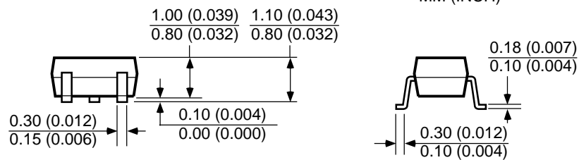
SC-70 (C5)
