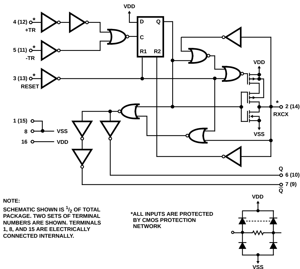
FIGURE 1. LOGIC DIAGRAM
