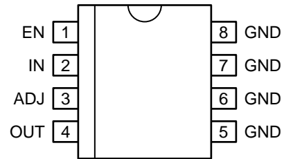
Adjustable MSOP-8 (MM)
