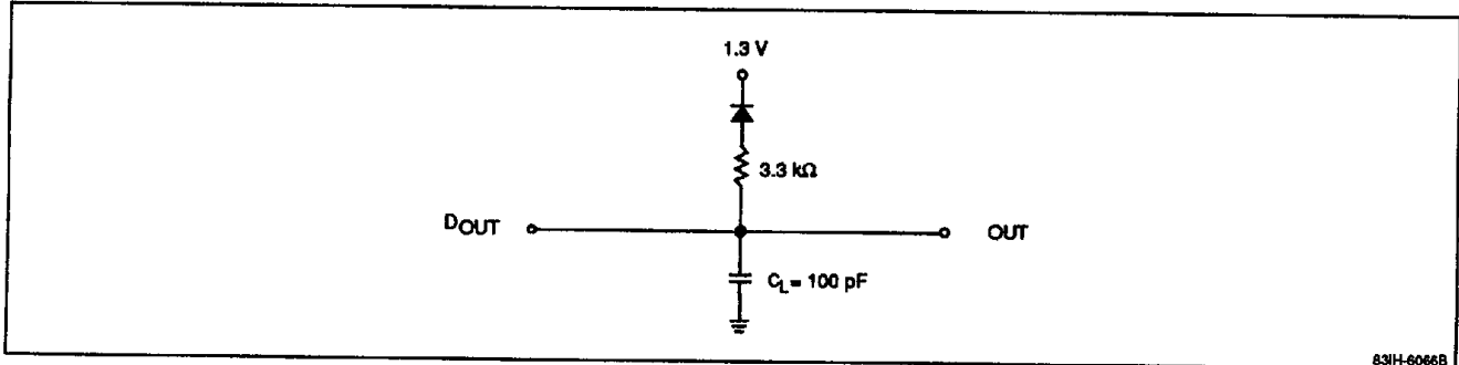
Figure 1. Output Load
