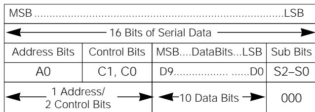
Figure 4. Serial-Data Format
