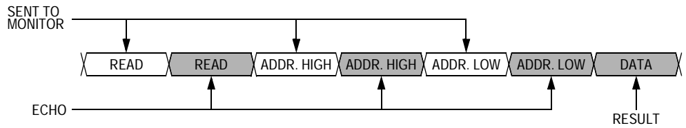
Figure 10-4. Read Transaction
