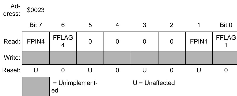
Figure 9-40. Fault Status Register (FSR)
