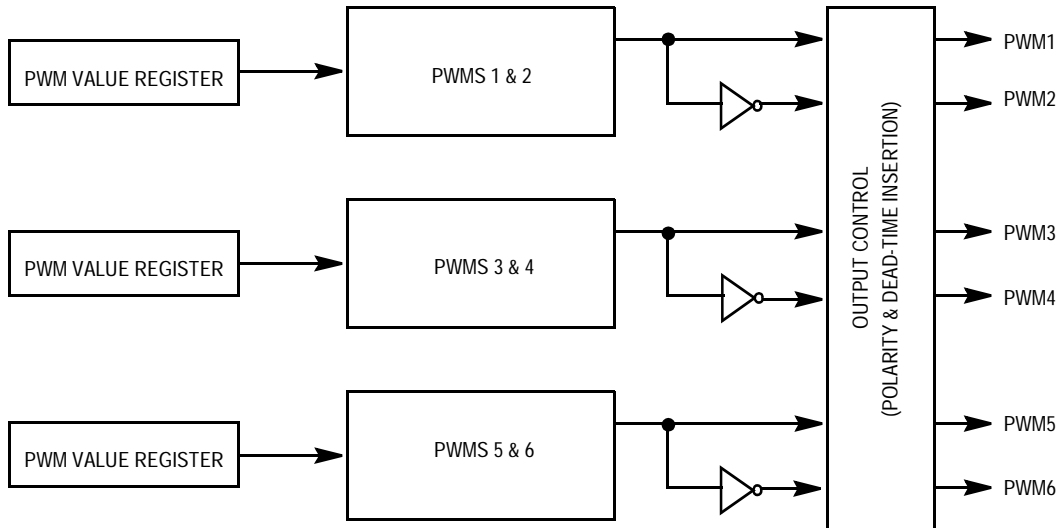
Figure 9-11. Complementary Pairing
