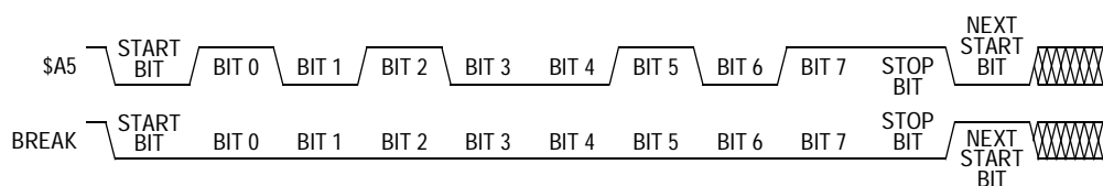
Figure 10-3. Sample Monitor Waveforms
