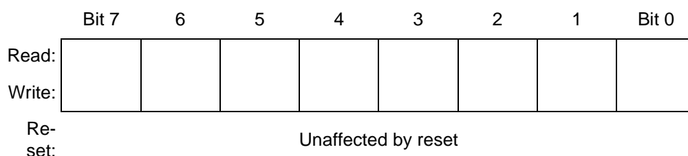
Figure 6-2. Accumulator (A)
