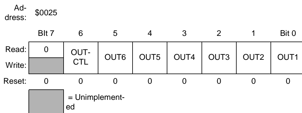
Figure 9-18. PWM Output Control Register (PWMOU)
