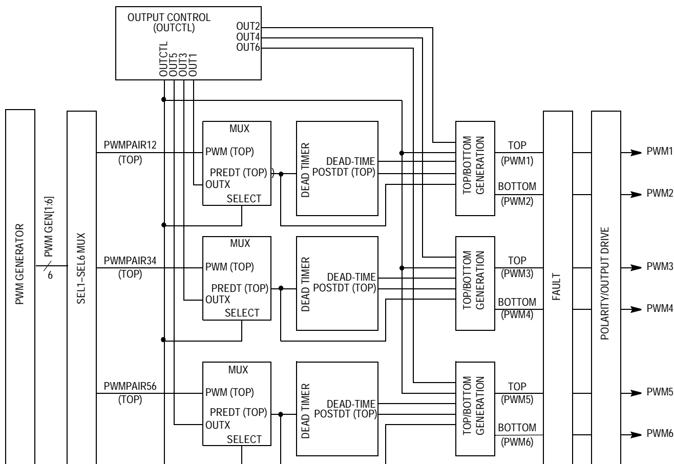
Figure 9-13. Dead-Time Generators
