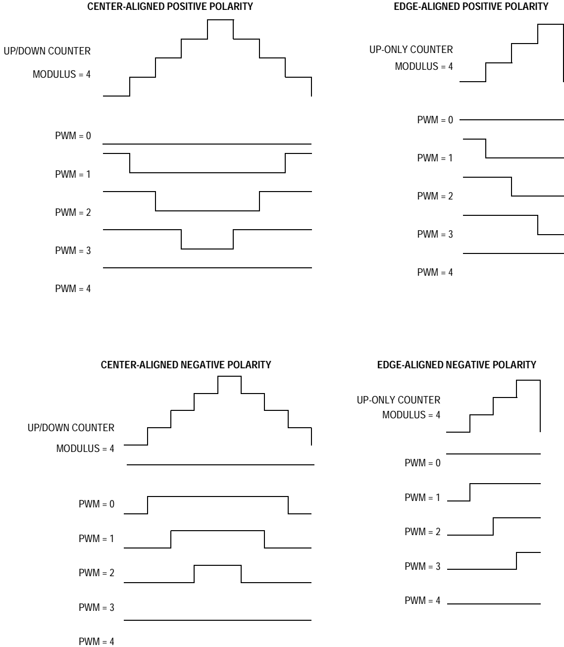
Figure 9-17. PWM Polarity
