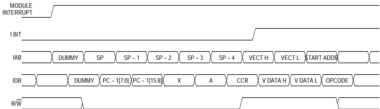
Figure 7-8. Interrupt Entry
