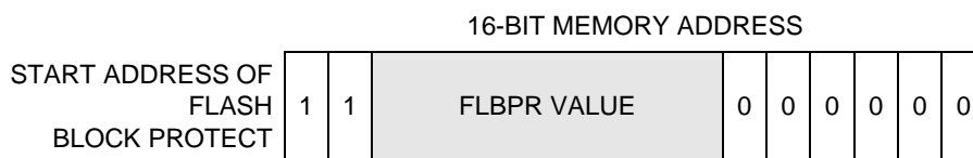
Figure 4-4. FLASH Block Protect Address
