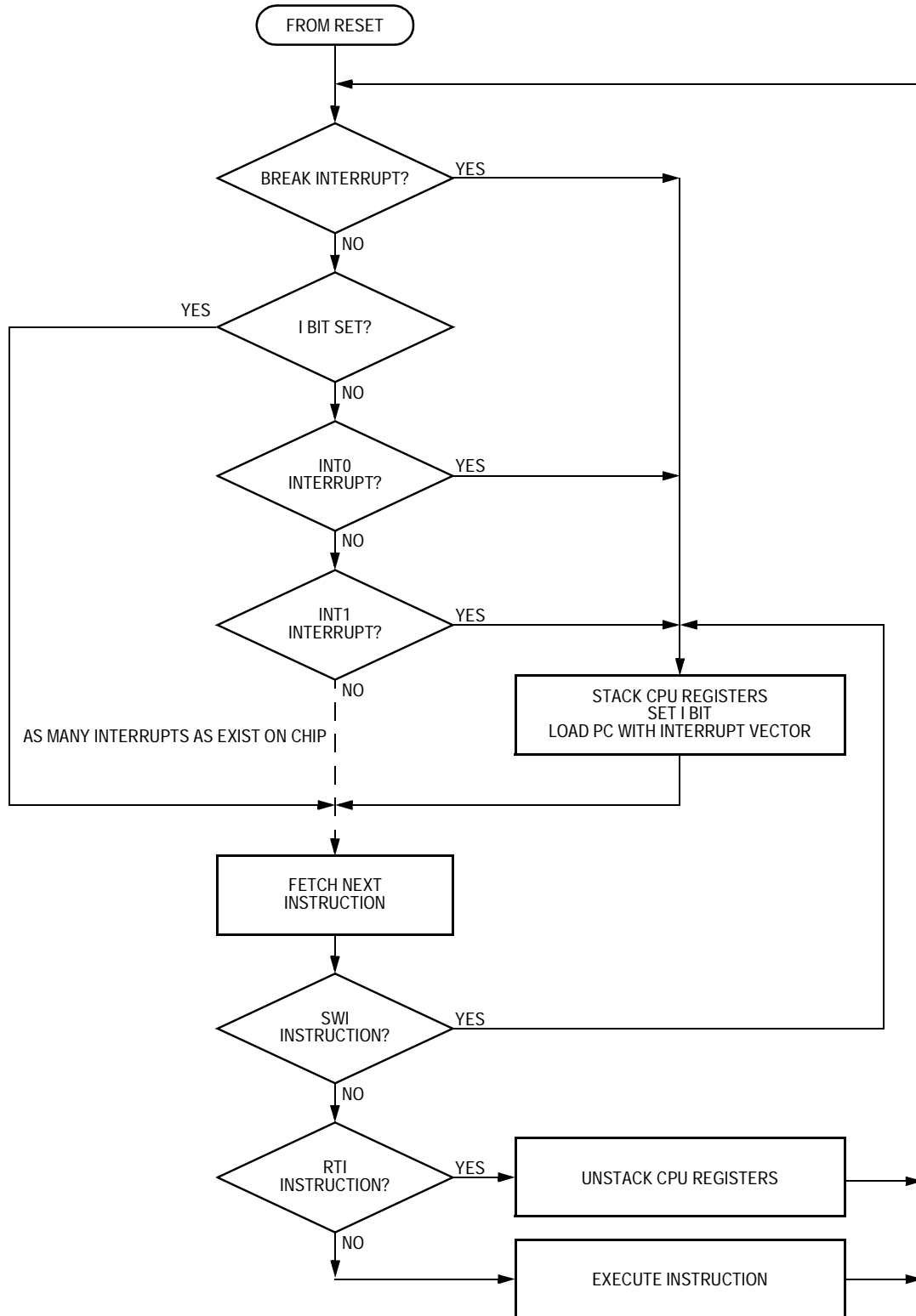
Figure 7-9. Interrupt Processing
