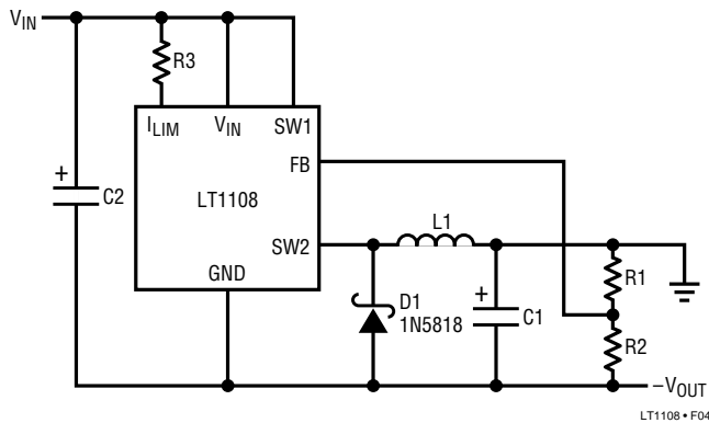
Figure 4. Positive-to-Negative Converter
