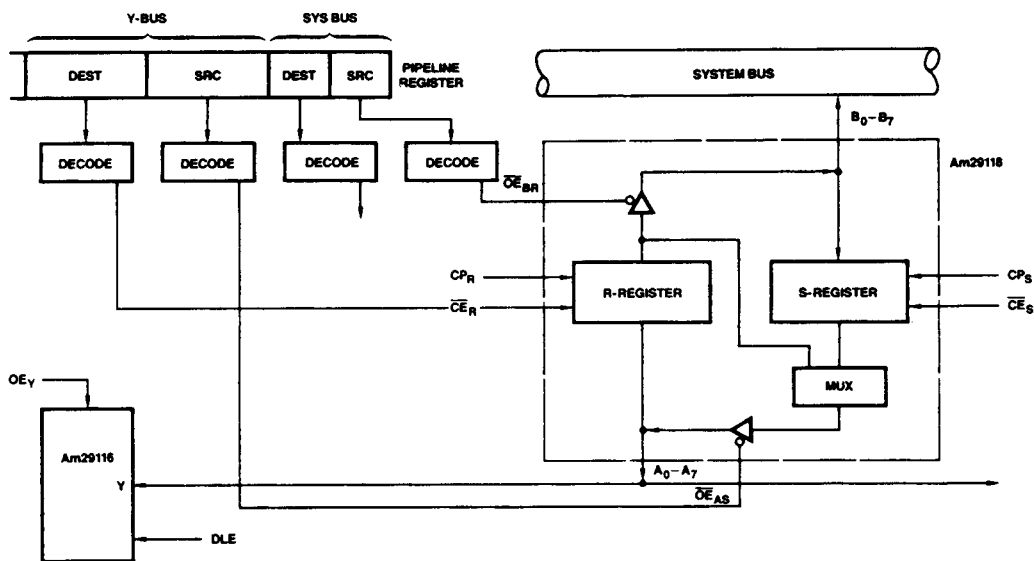
Figure 2. System Configuration.
