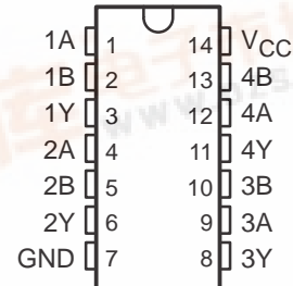
SN54AHCT08 ... J OR W PACKAGE SN74AHCT08 ... D, DB, DGV, N, OR PW PACKAGE (TOP VIEW)
