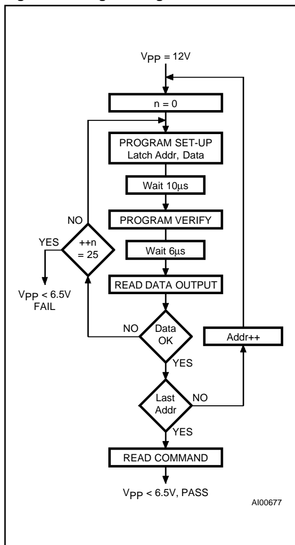
Figure 13. Programming Flowchart
