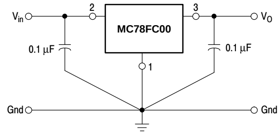
Figure 6. Typical Application
