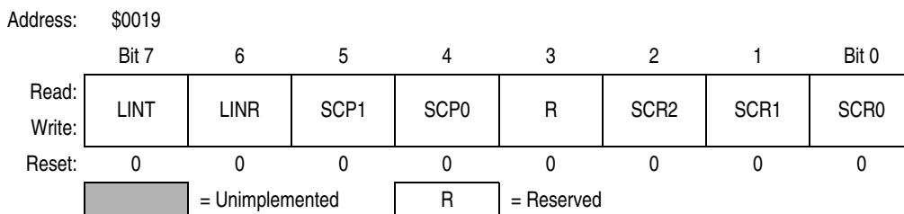
Figure 15-17. ESCI Baud Rate Register (SCBR)
