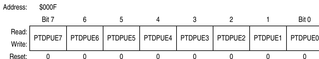
Figure 13-16. Port D Input Pullup Enable Register (PTDUE)
