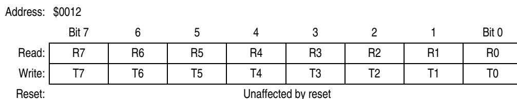
Figure 17-16. SPI Data Register (SPDR)
