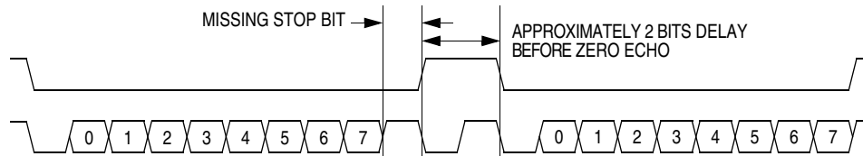
Figure 20-12. Break Transaction
