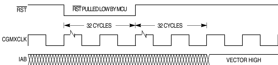
Figure 16-5. Internal Reset Timing
