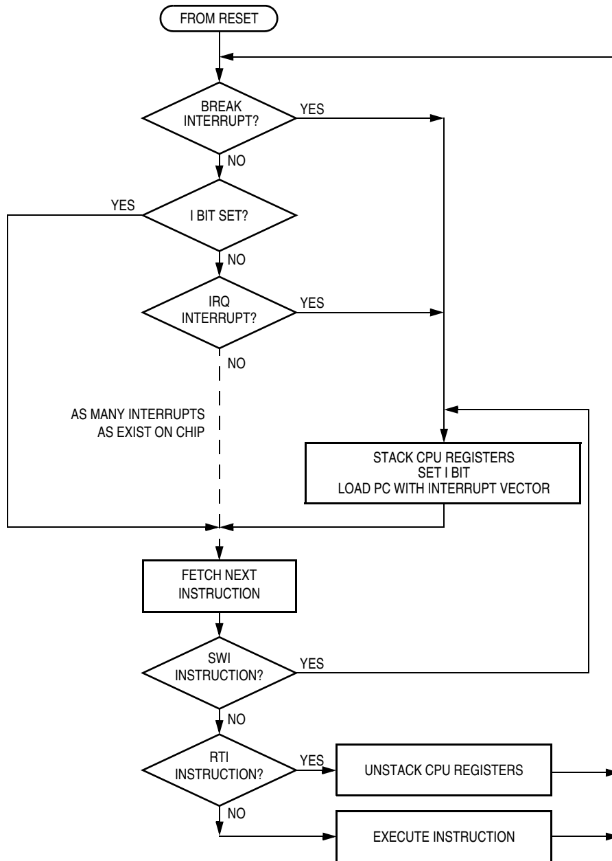
Figure 16-10. Interrupt Processing
