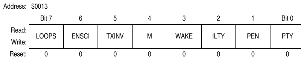
Figure 15-10. ESCI Control Register 1 (SCC1)
