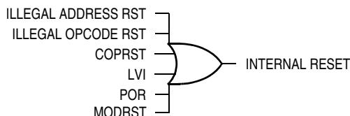
Figure 16-6. Sources of Internal Reset
