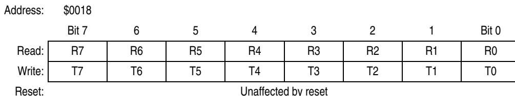
Figure 15-16. ESCI Data Register (SCDR)
