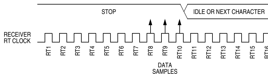
Figure 15-9. Fast Data
