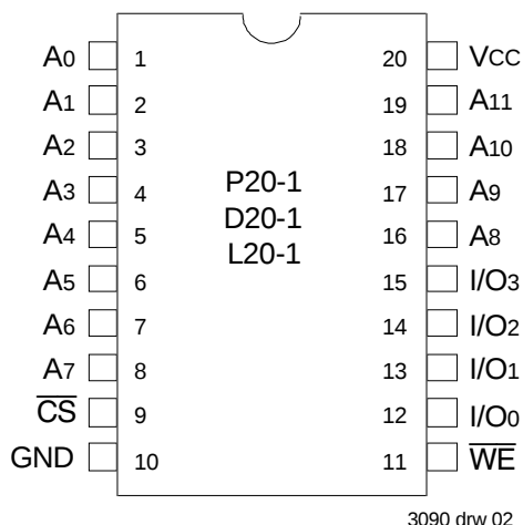
DIP/LCC Top View
