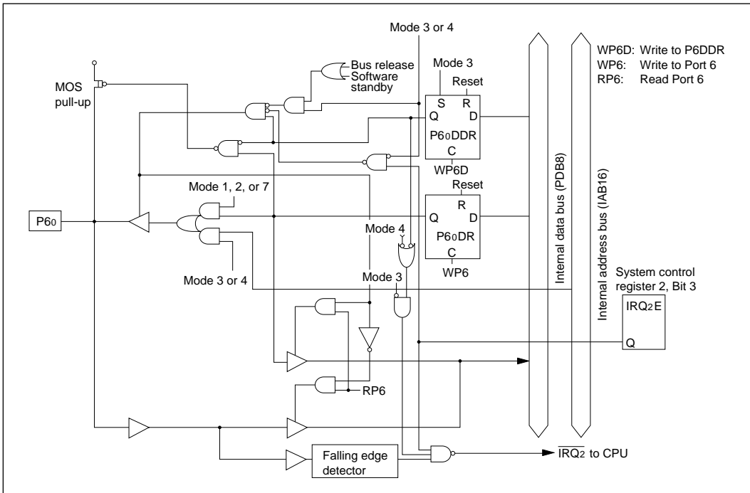
Figure C-6 (a) Schematic Diagram of Port 6, Pin P60
