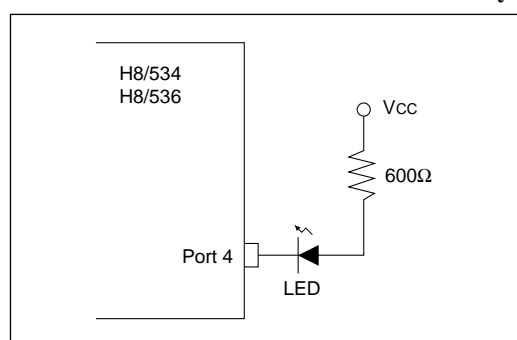
Figure 20-2 Example of Circuit for Driving an LED
