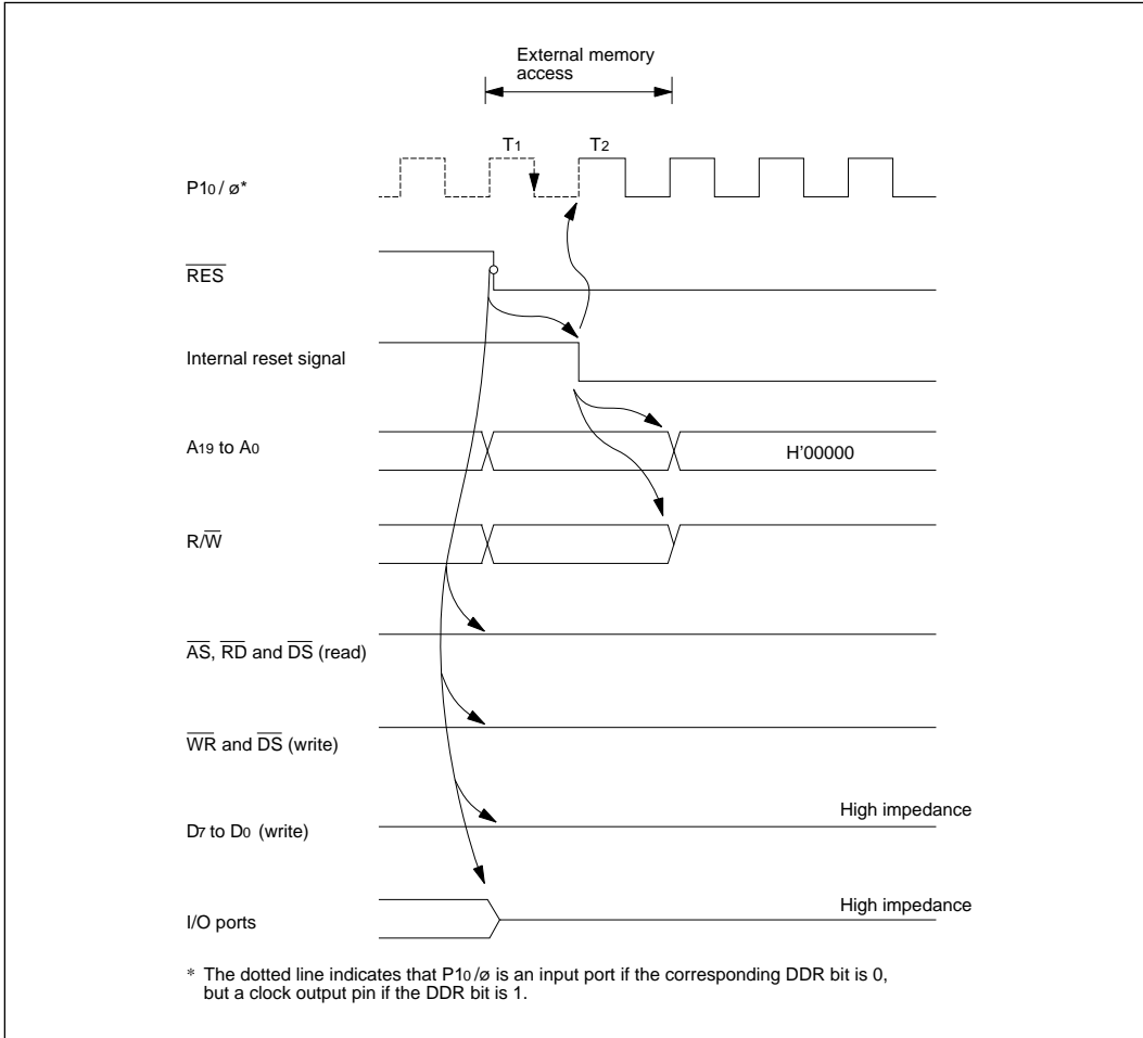
Figure E-3 Reset during Memory Access (Mode 3)
