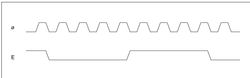
Figure 8-7 Phase Relationship of \phi Clock and E Clock
