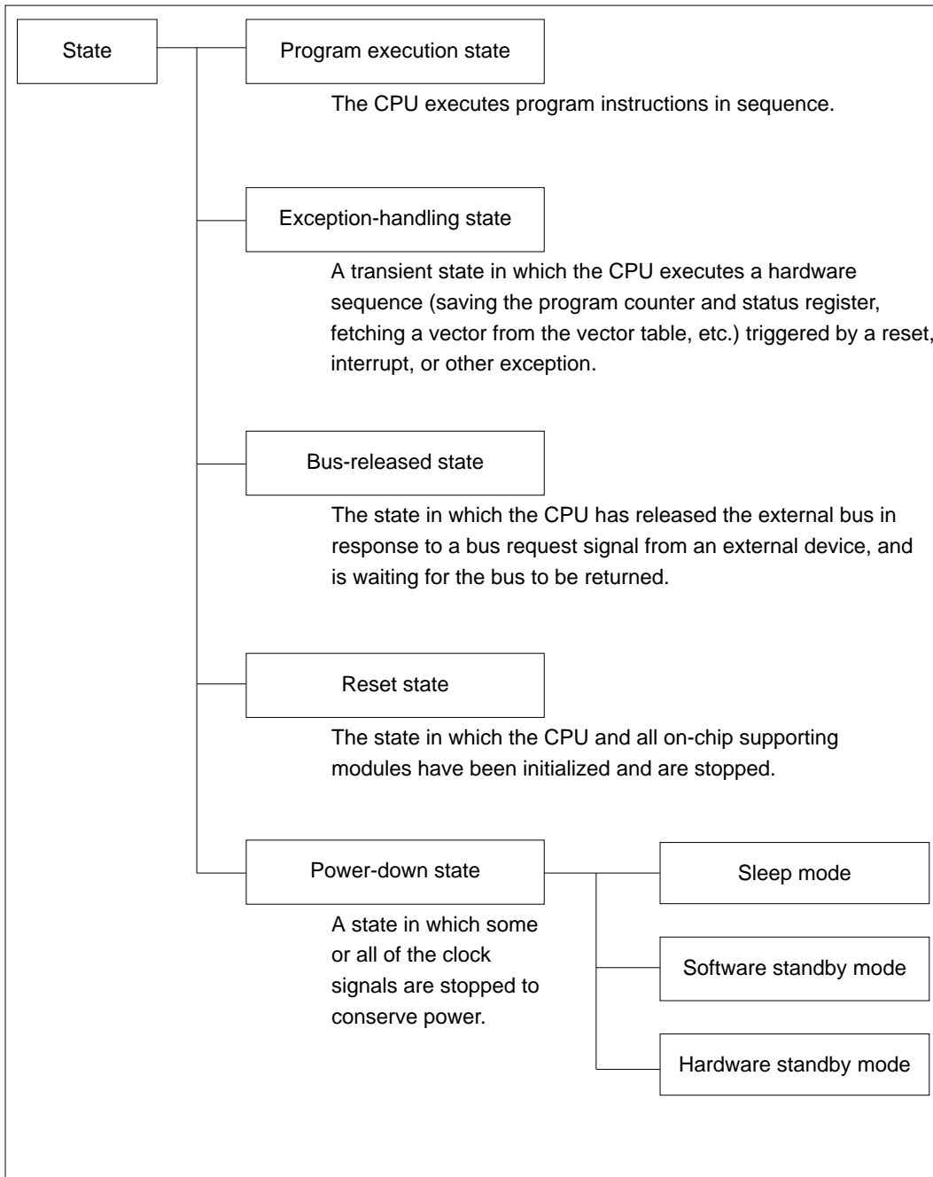
Figure 3-11 Operating States
