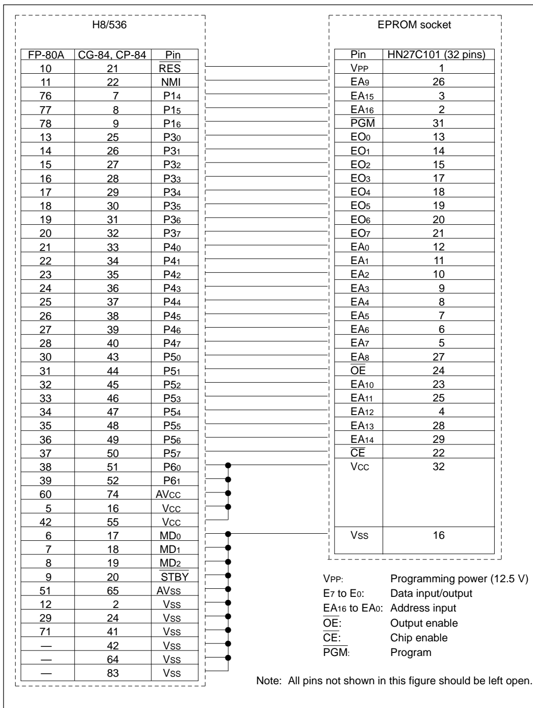
Figure 17-2(b) Socket Adapter Pin Arrangements (H8/536)
