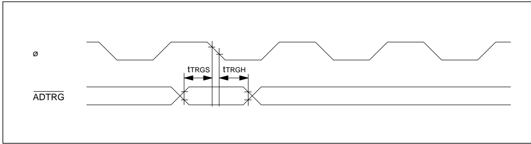
Figure 20-22 A/D Trigger Signal Input Timing
