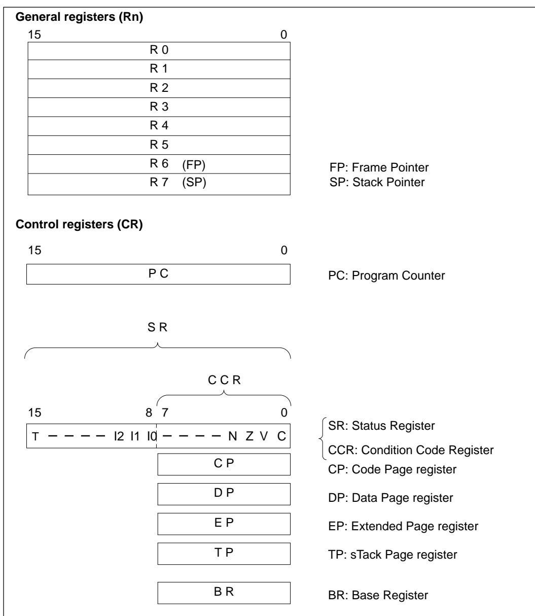
Figure 3-2 Registers in the CPU
