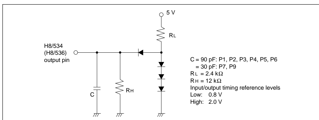
Figure 20-3 Output Load Circuit
