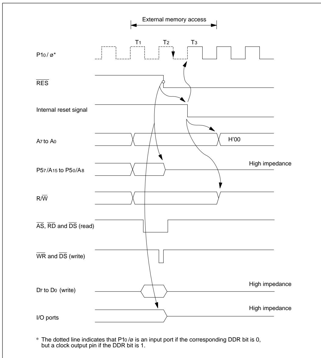
Figure E-2 Reset during Memory Access (Mode 2)
