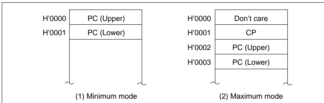
Figure 4-2 Reset Vector
