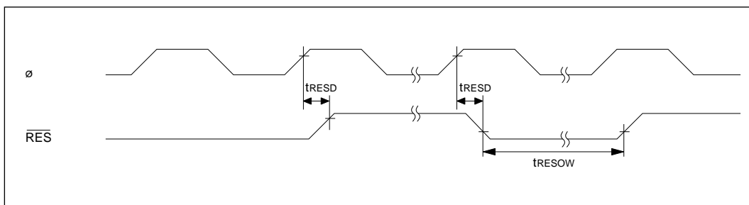
Figure 20-8 Reset Output Timing
