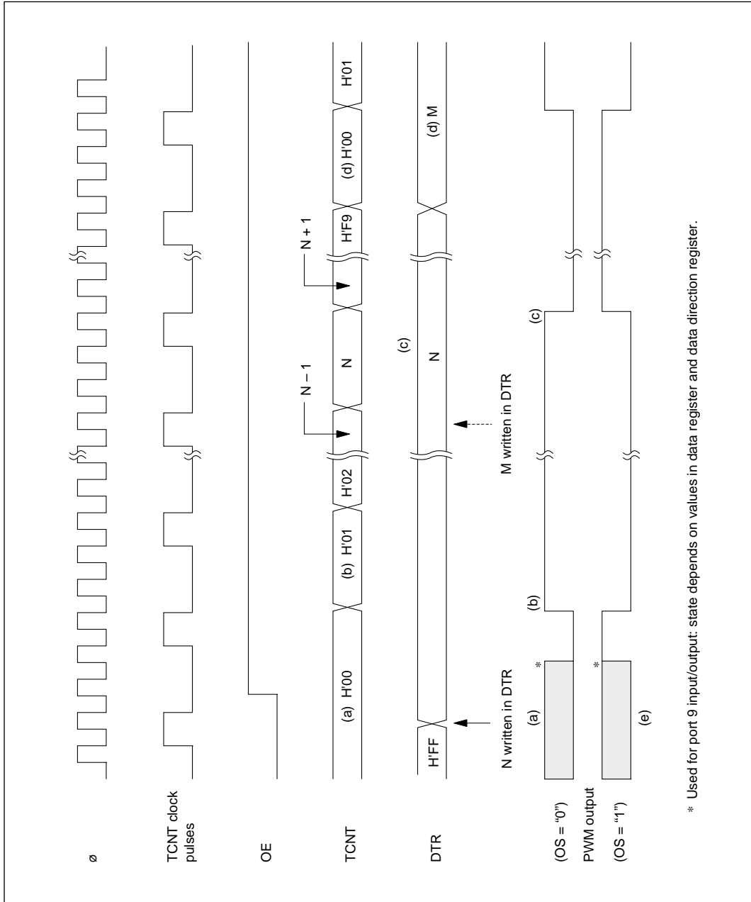
Figure 12-2 PWM Timing
