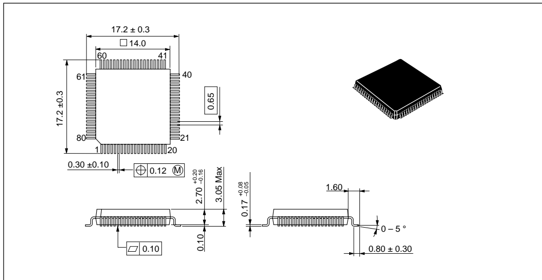
Figure G-3 Package Dimensions (FP-80A)
