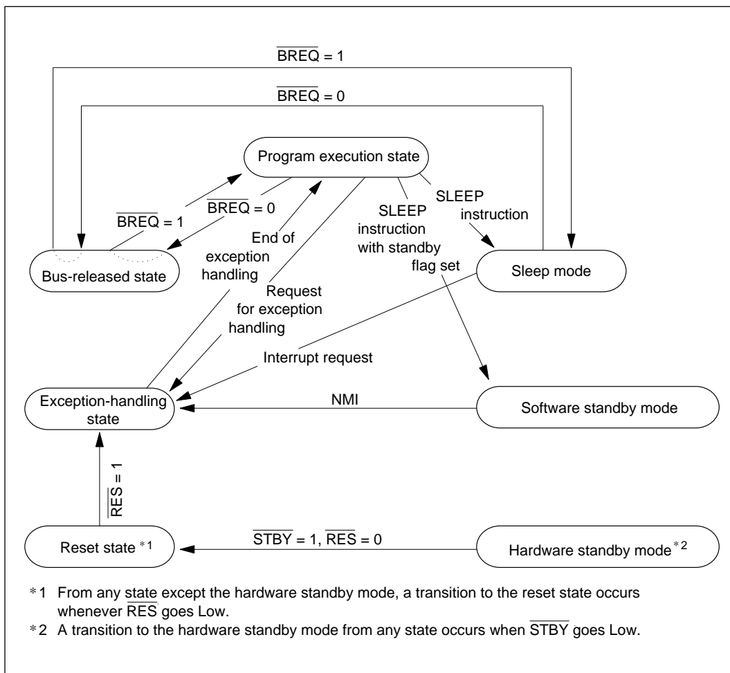
Figure 3-12 State Transitions
