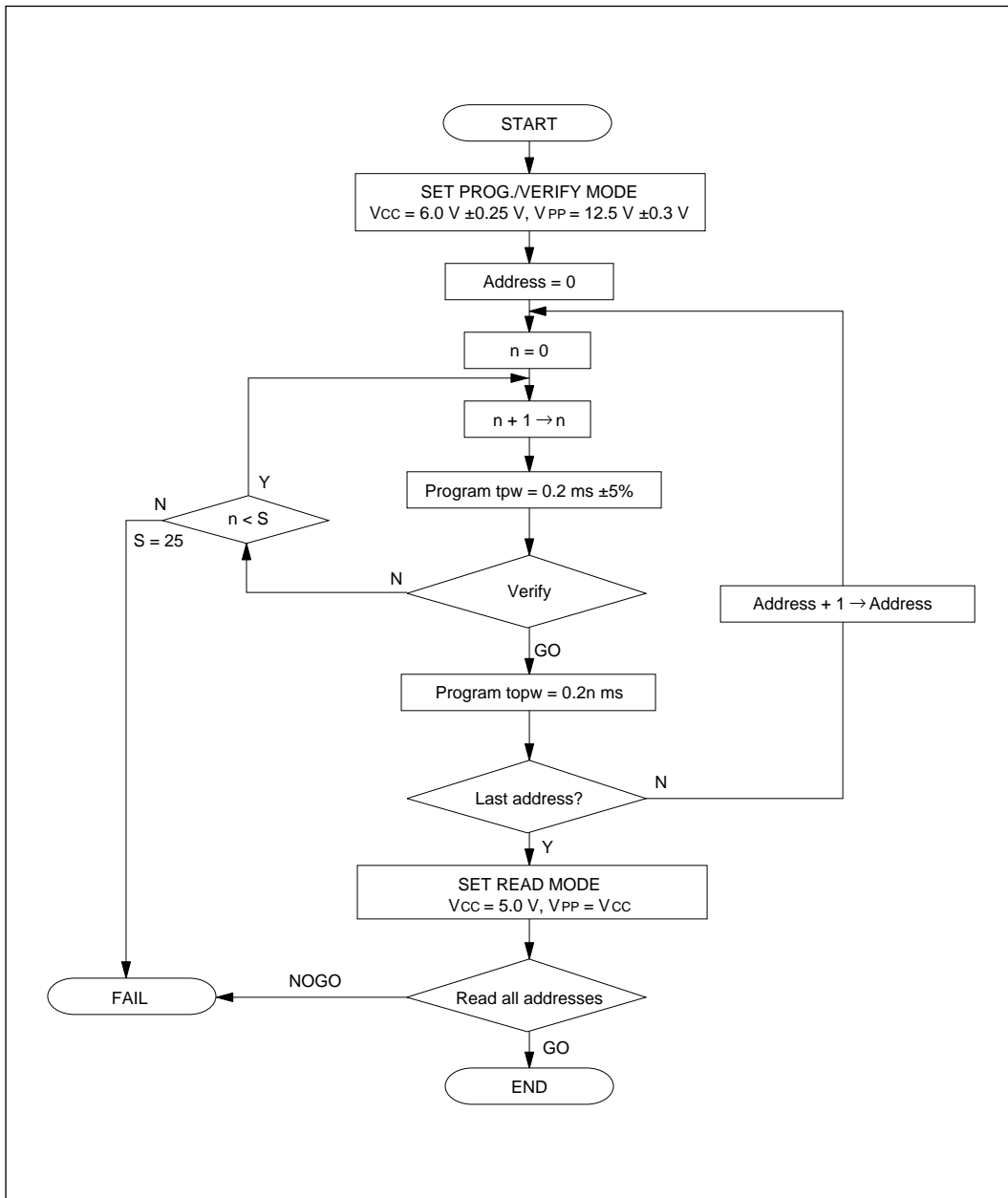
Figure 17-6 High-Speed Programming Flowchart (H8/536)
