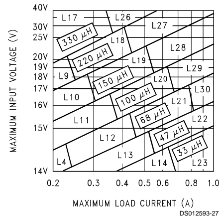
FIGURE 6. LM2598-12
