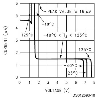
Shutdown/Soft-start Current
