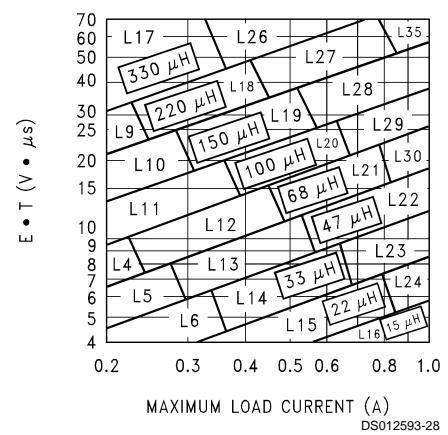
FIGURE 7. LM2598-ADJ
