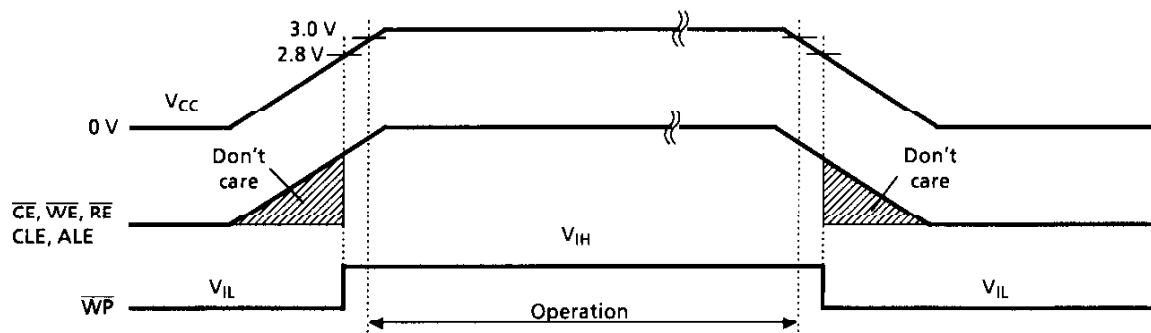
Figure 21. Power-on/off Sequence
