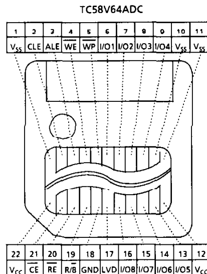
Figure 1. Pinout
