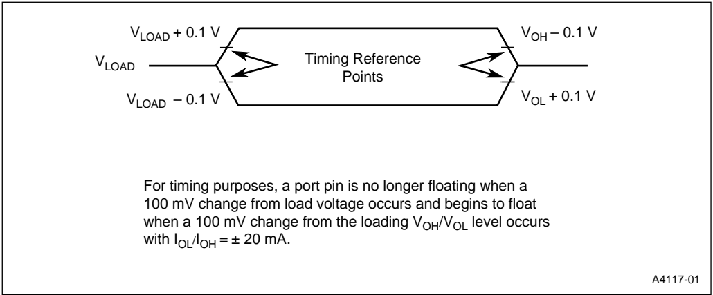
Figure 20. Float Waveforms
