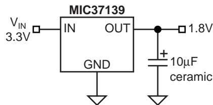
1.8V/1.5A Regulator
