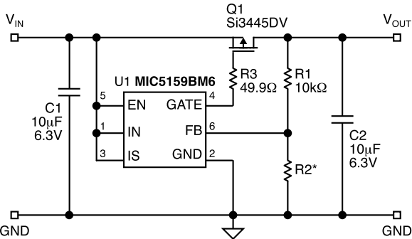
Application Circuit
