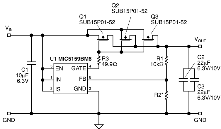
Application Circuit
