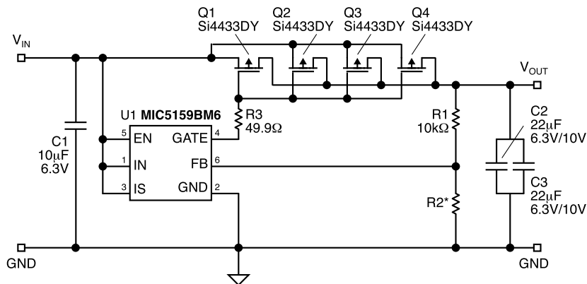
Application Circuit
