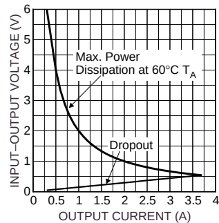
SUB15P01-52 SOA
