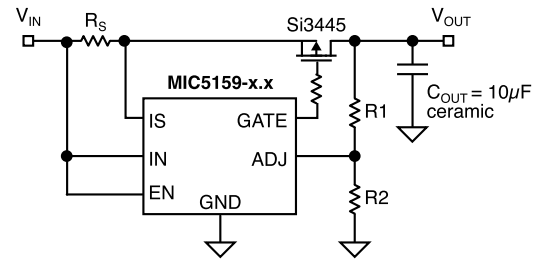
Figure 4. Adjustable Regulator Design
