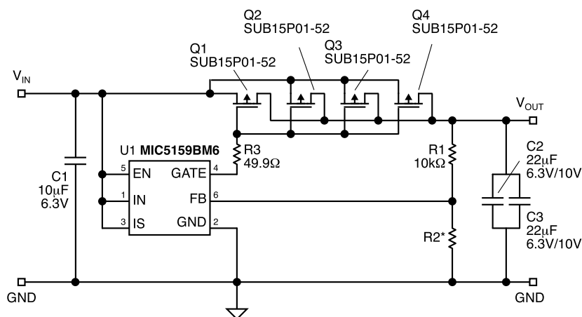
Application Circuit
