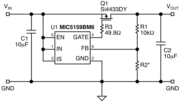
Application Circuit
