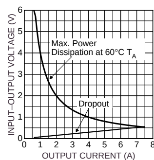
SUB15P01-52 x2 SOA
