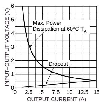
SUB15P01-52 x4 SOA
