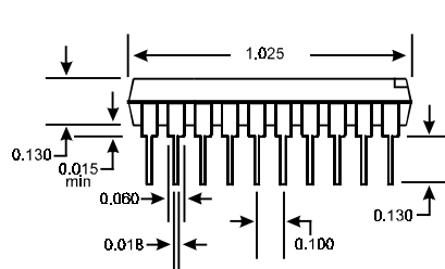
20-Pin DIP Package
