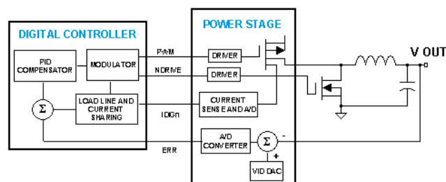
DIGITAL BLOCK DIAGRAM
