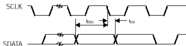
FIGURE 7. DATA READ TIMING
