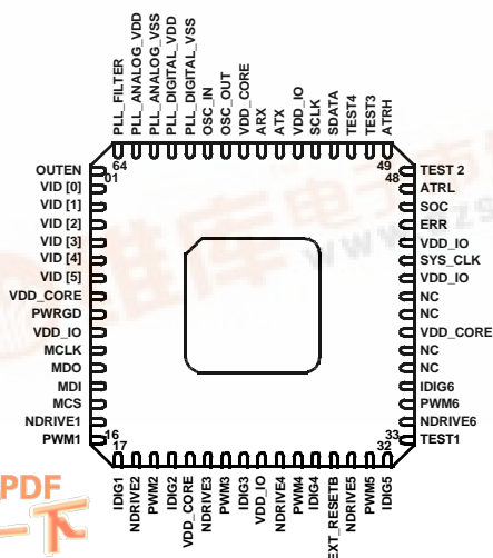
ISL6590 (QFN) TOP VIEW
