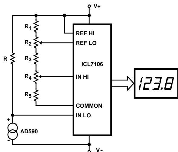
FIGURE 11. BASIC DIGITAL THERMETER, CELSIUS AND FAHRENHEIT SCALES
