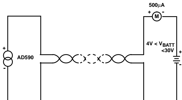
FIGURE 10. SIMPLEST THERMOMETER
