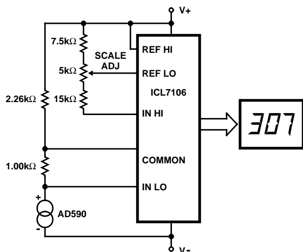
FIGURE 12. BASIC DIGITAL THERMETER, KELVIN SCALE
