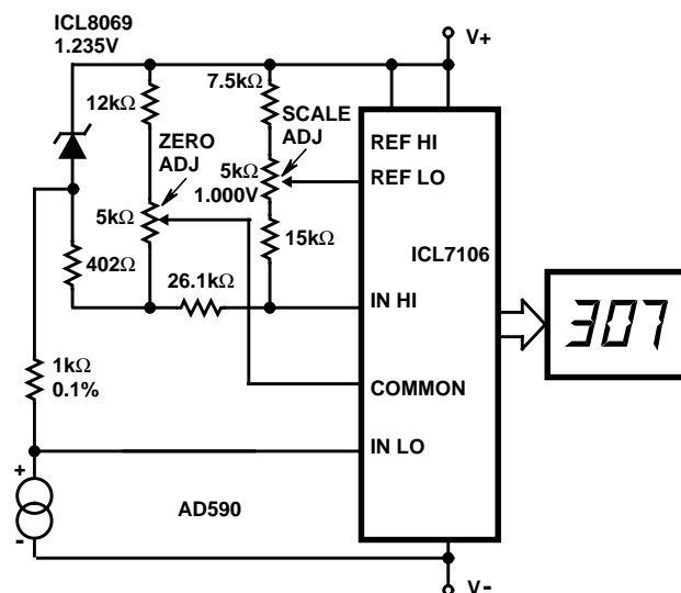
FIGURE 13. BASIC DIGITAL THERMETER, KELVIN SCALE WITH ZERO ADJUST
