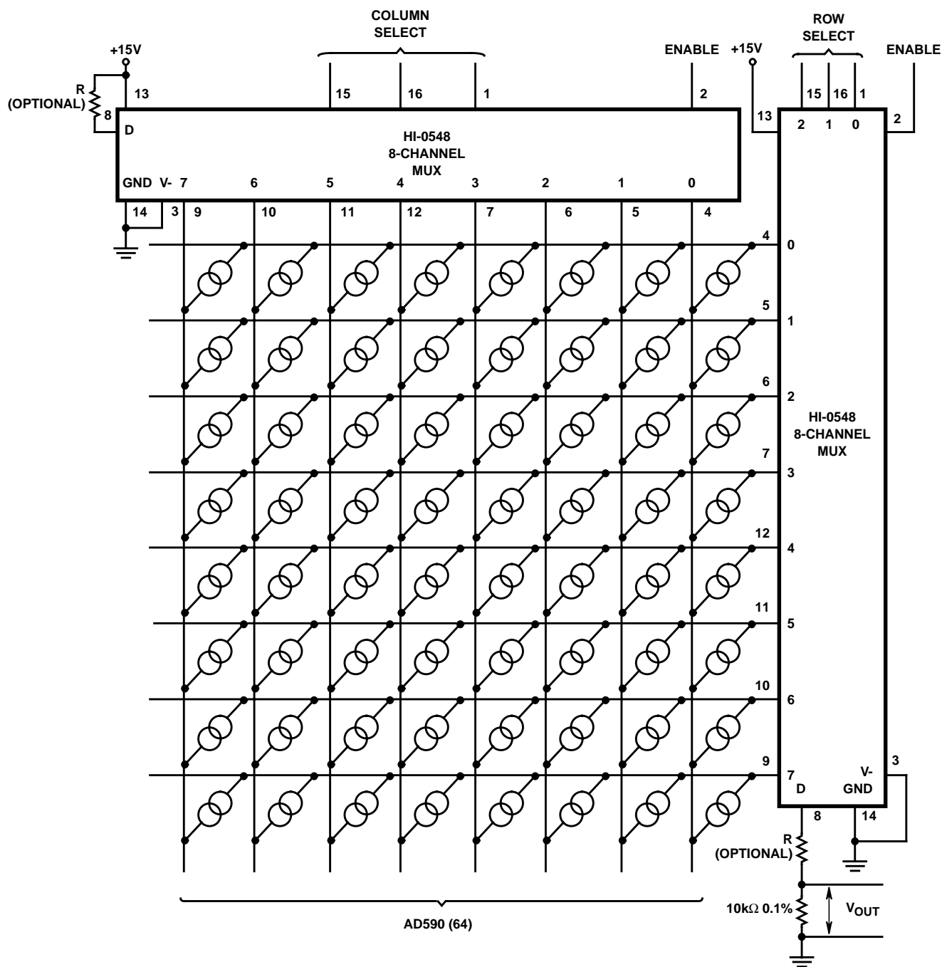
FIGURE 17. MULTIPLEXING SENSORS
