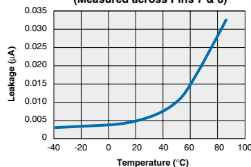
TS190L Typical Leakage vs. Temperature (Measured across Pins 7 & 8)
