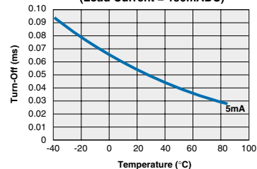
TS190L Typical Turn-Off vs. Temperature (Load Current = 150mADC)
