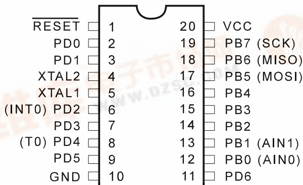
PDIP/SOIC/SSOP
