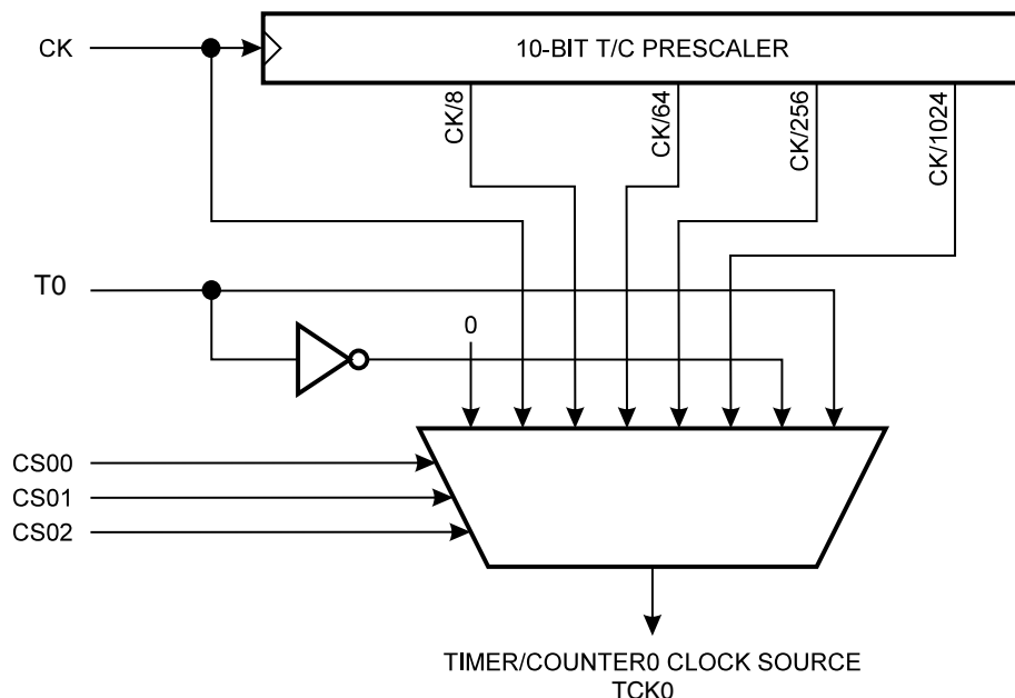
Figure 18. Timer/Counter0 Prescaler
