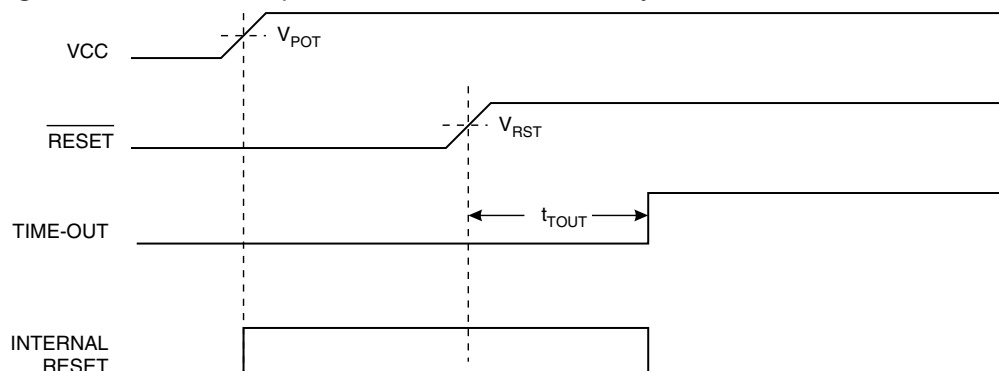
Figure 15. MCU Start-up, \overline{\text{RESET}} Controlled Externally
