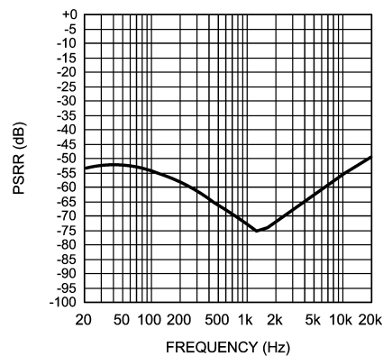
Power Supply Rejection Ratio V_{DD} = 1.5V, V_{RIPPLE} = 200mV_{PP} R_L = 16\Omega, \text{Single Ended Output} Input Terminated into 10\Omega
