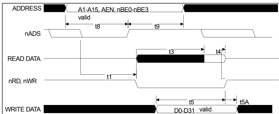
FIGURE 17 - ASYNCHRONOUS CYCLE - USING nADS
