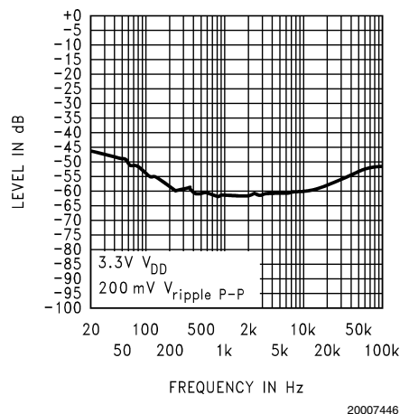
Power Supply Rejection Ratio (PSRR) @ V_{DD} = 3.3V
