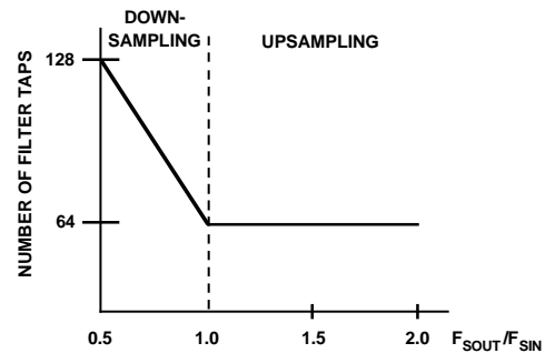
Figure 8. Number of Filter Taps as a Function of F_{\text{SOUT}}/F_{\text{SIN}}
