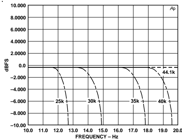
Figure 19. AD1890/AD1891 Digital Filter Signal Transfer Function, 10 kHz to 20 kHz, 44.1 kHz Input Sample Frequency, 40, 35, 30 and 25 kHz Output Sample Frequencies
