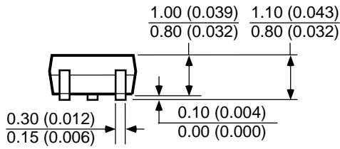
SC-70 (C5)
