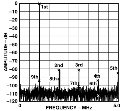
FIGURE 4. TYPICAL FFT, f_{IN} = 1.0 MHz (INPUT SPAN = 5V, V_{CM} = 2.5V )
