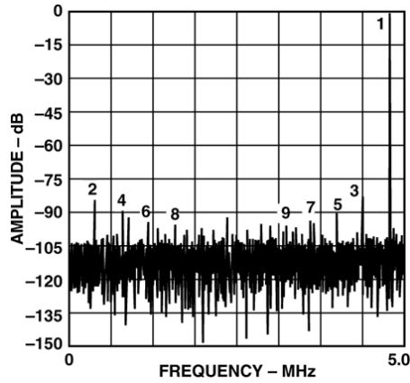
FIGURE 7. TYPICAL FFT, f_{IN} = 5.0 \text{ MHz} (INPUT SPAN = 2 V, V_{CM} = 2.5 \text{ V} )
