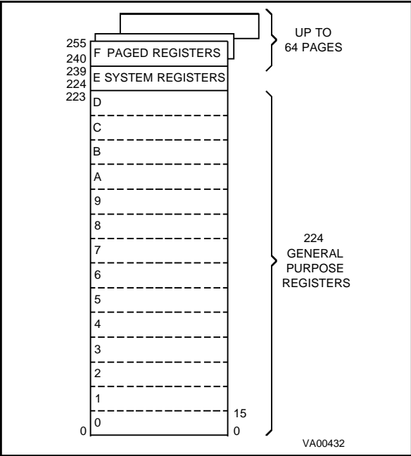
Figure 1-5. Register Grouping
