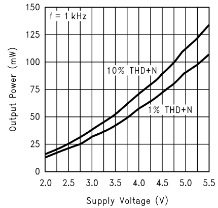
Output Power vs Supply Voltage Headphone Output, R_L = 32\Omega
