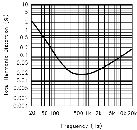
THD+N vs Frequency at V DD = 5V, R L = 32Ω, PWR = 70mW, Headphone mode
