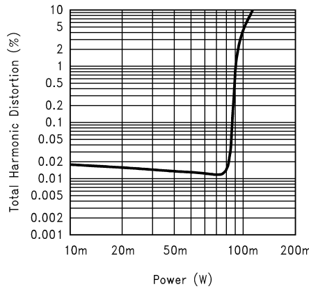
THD+N vs Power Out at V DD = 5V, R L = 32Ω, 1kHz, Headphone mode
