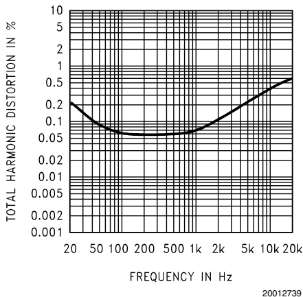
THD+N vs Frequency at V_{DD} = 2.6V , 8\Omega R_L , and PWR = 100mW
