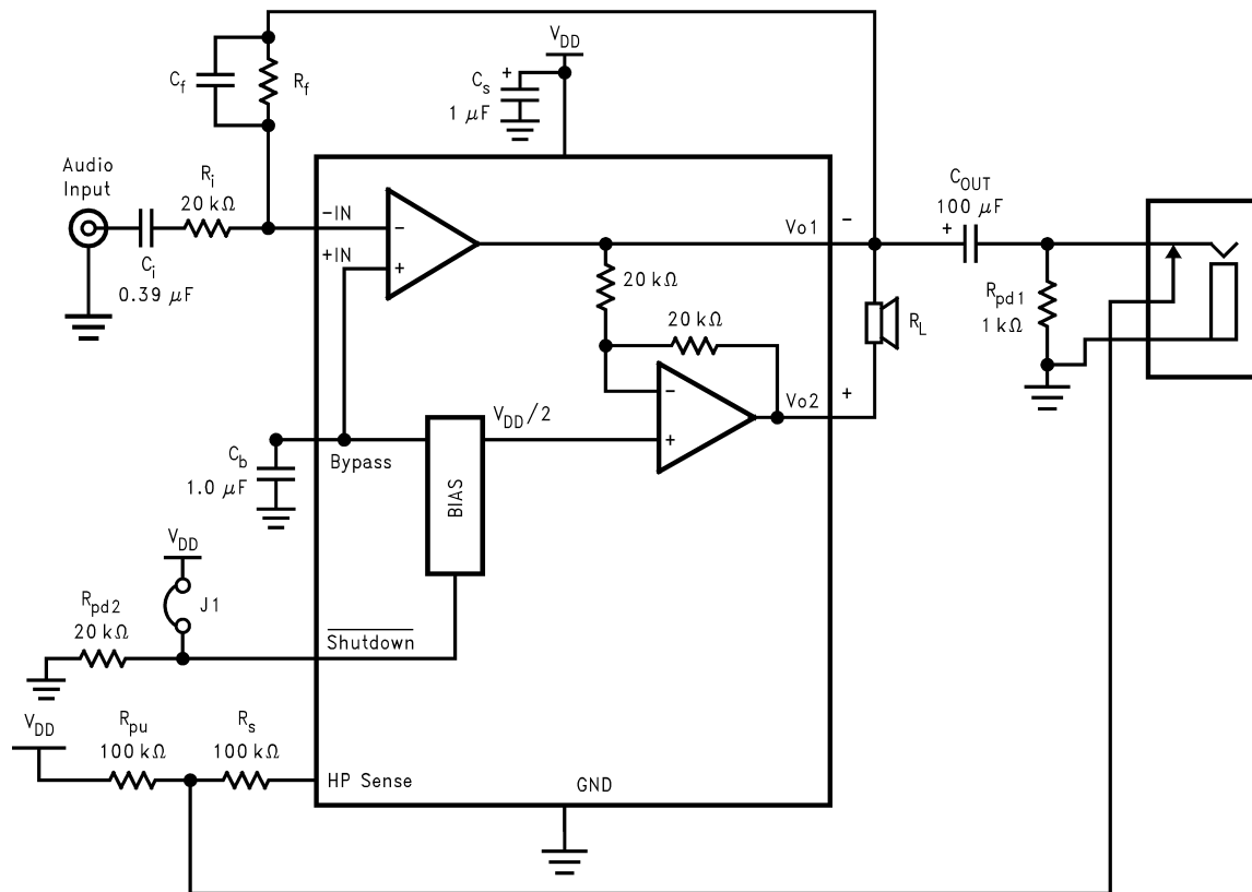
FIGURE 3. Higher Gain Audio Amplifier
