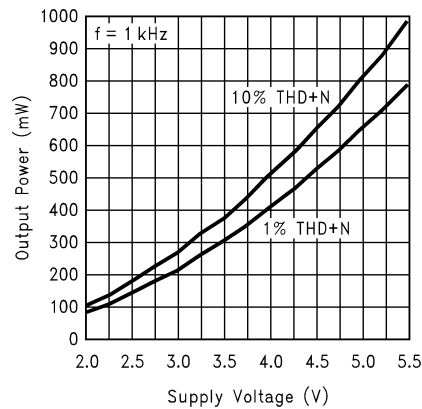
Output Power vs Supply Voltage R L = 16Ω
