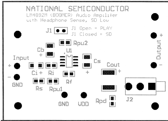
Silk Screen
