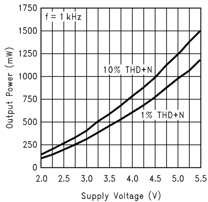
Output Power vs Supply Voltage R L = 8Ω
